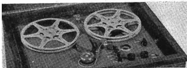
(Brush Paper) Home-type magnetic recorder using coated paper.
