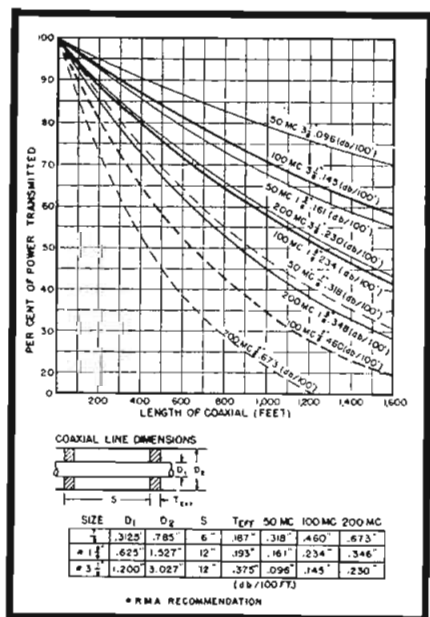
(Holtz Paper) Plot of coaxial line efficiency of turnstile antenna.
