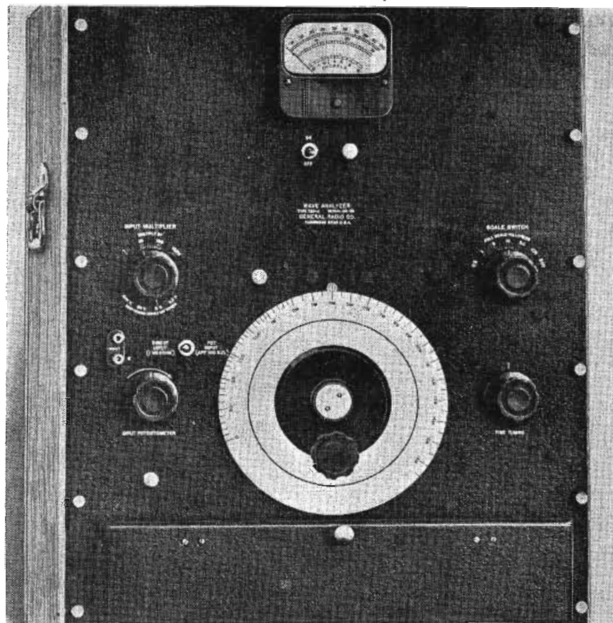
A heterodyne-type wave analyzer. (G.R. 736-A)
