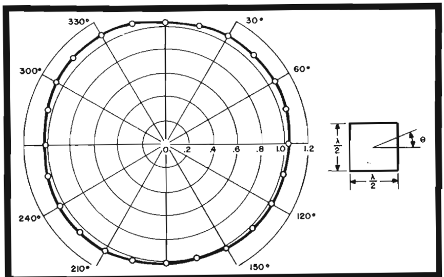
(Kandorian Paper) Measured horizontal pattern of square loop f-m antenna.
