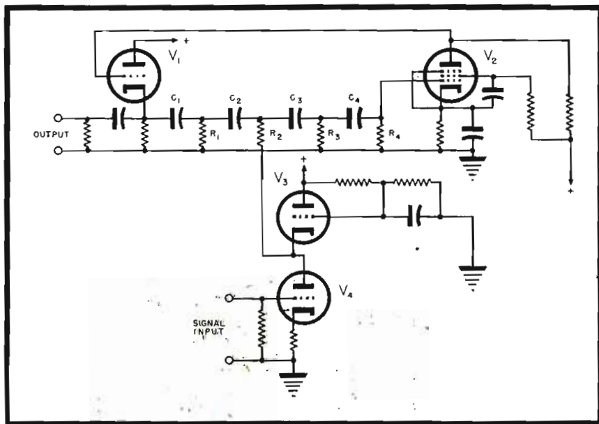
Figure 8 A ladder-network RC oscillator employing a four-step ladder and tubes V_1 and V_4 to vary the frequency.
