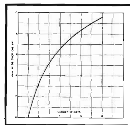
(Scheldorf Paper) Gain characteristics for multiple bays of circular antenna.
