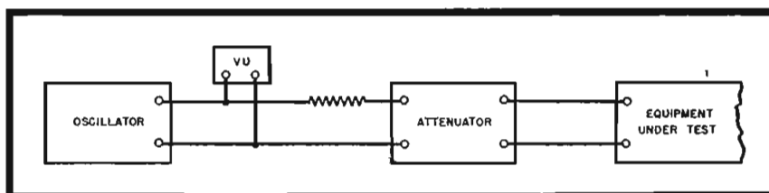
Figure 1 Conventional means of coupling test oscillator to transmitter.
